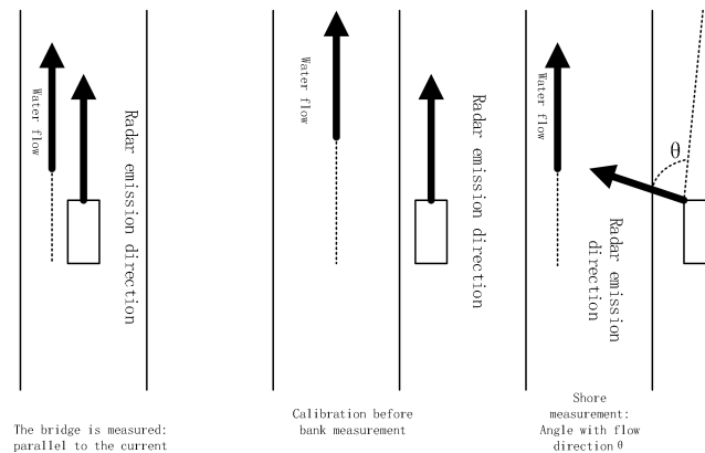
FIG. 21 Schematic diagram of the horizontal angle of radar waves
