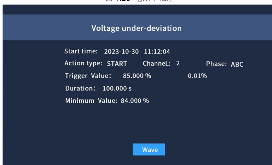
Fig. 4.28 Voltage under-deviation
