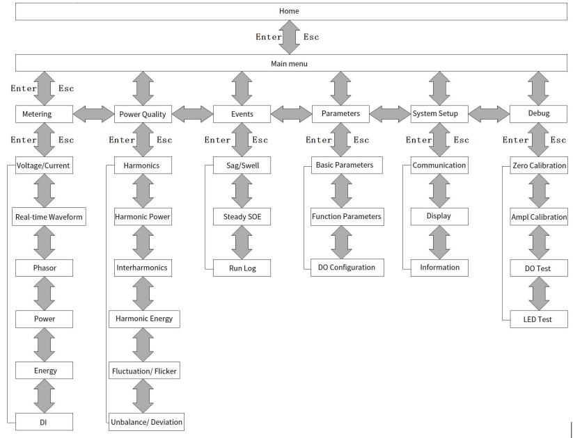
Fig. 4.2 Quick navigation
