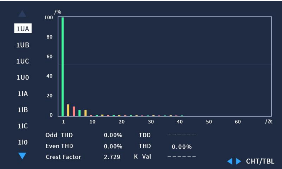
Fig. 4.13 Harmonics Chart
