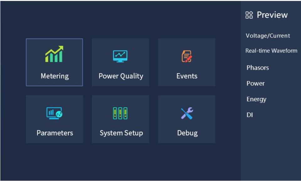
Fig. 4.4 Main Menu
