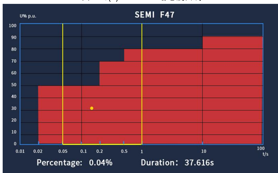
Fig. 4.26(b) SEMI F47 Curves
