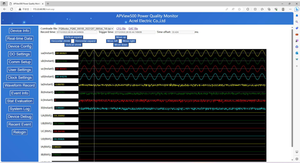
Fig. 1.4 Waveform Screen
