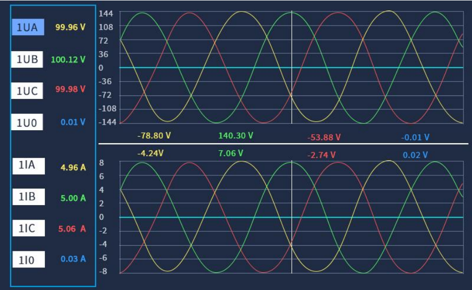
Fig. 4.7 Real-time Waveform
