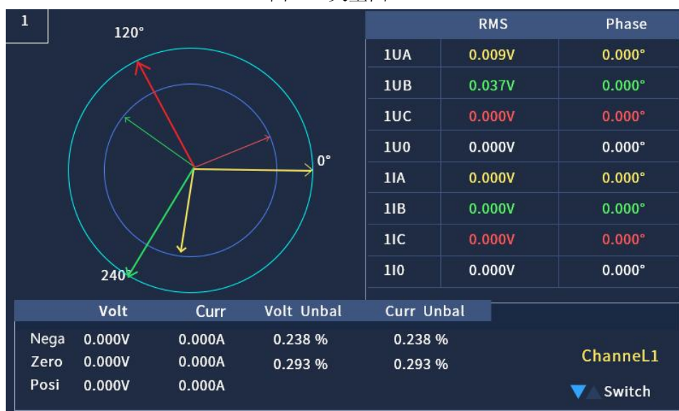
Fig. 4.8 Phasors
