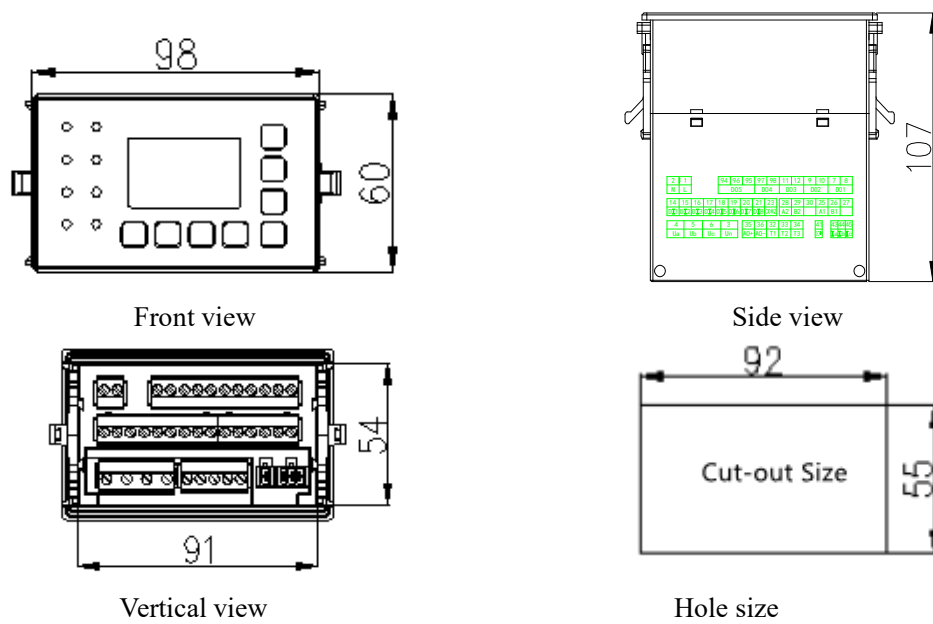
Figure 4 Panel size of split protector ARD2M
