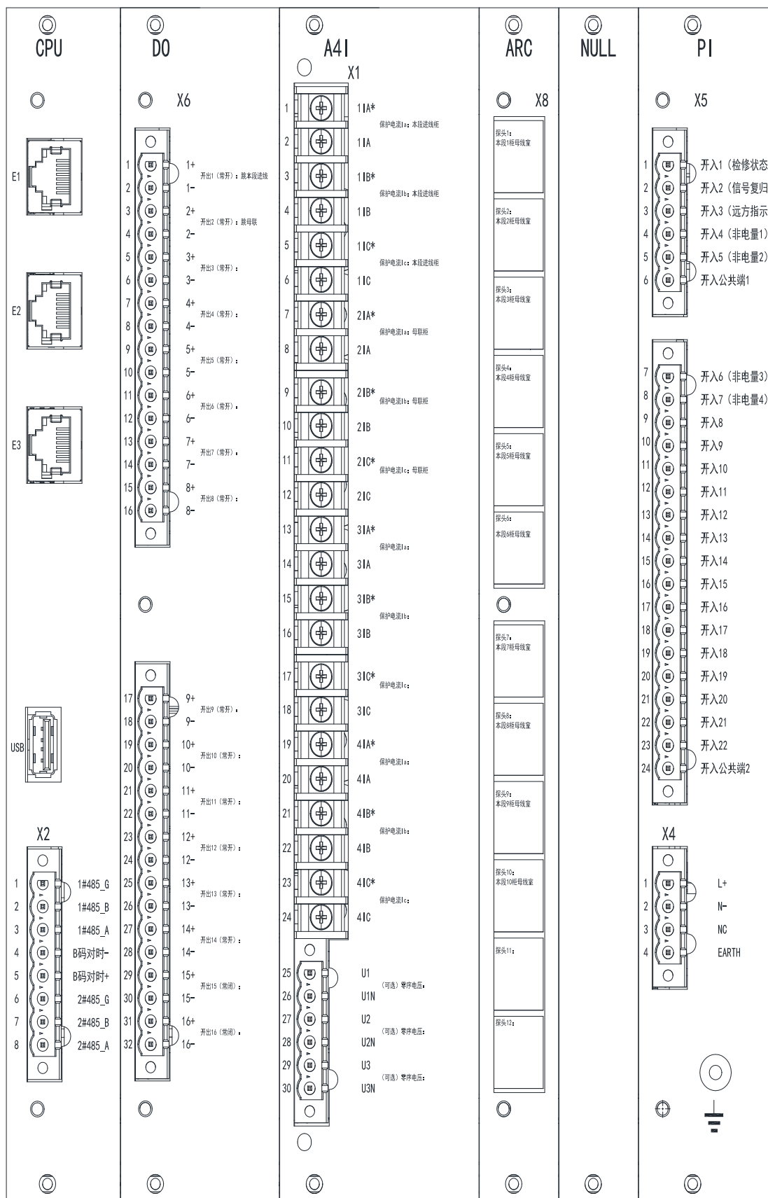
图 1.2 示例一背板端子接线示意图 Figure 1.2 Example 1 Backboard Terminal Wiring Diagram
