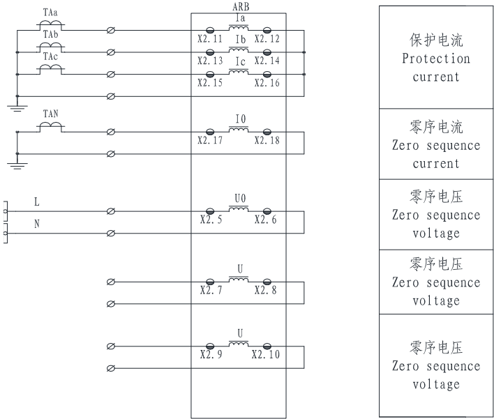
图 3.2 电流、电压回路二次原理图 Figure 3.2 Secondary schematic diagram of current and voltage circuits
