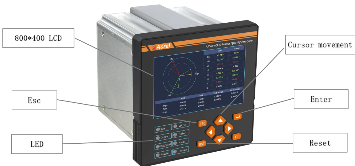
Fig. 4.1 Front Panel
