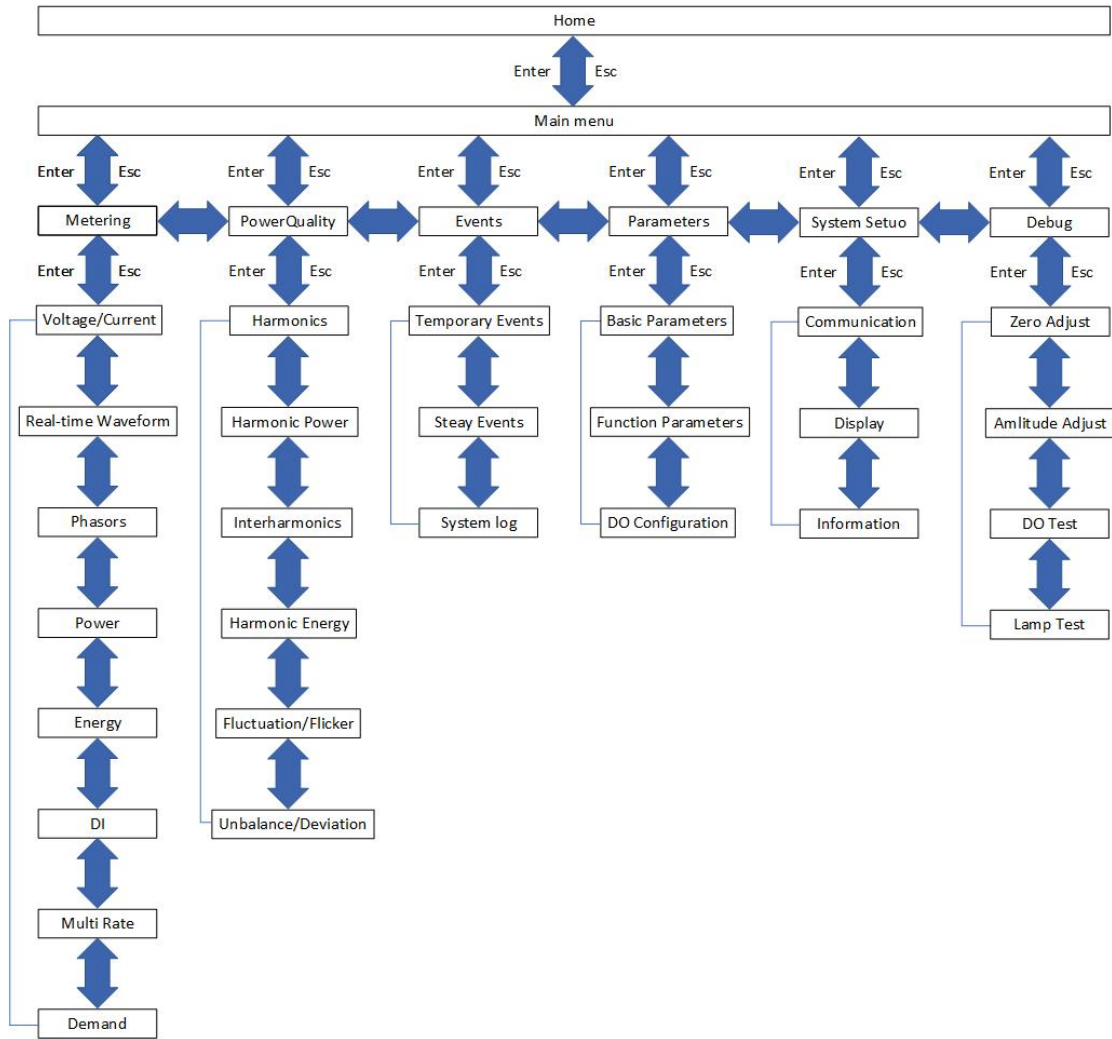
Fig. 4.2 Quick navigation
