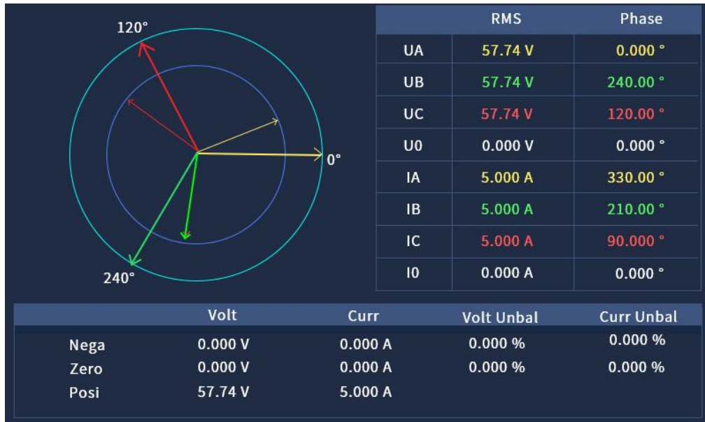
Fig. 4.8 Phasors
