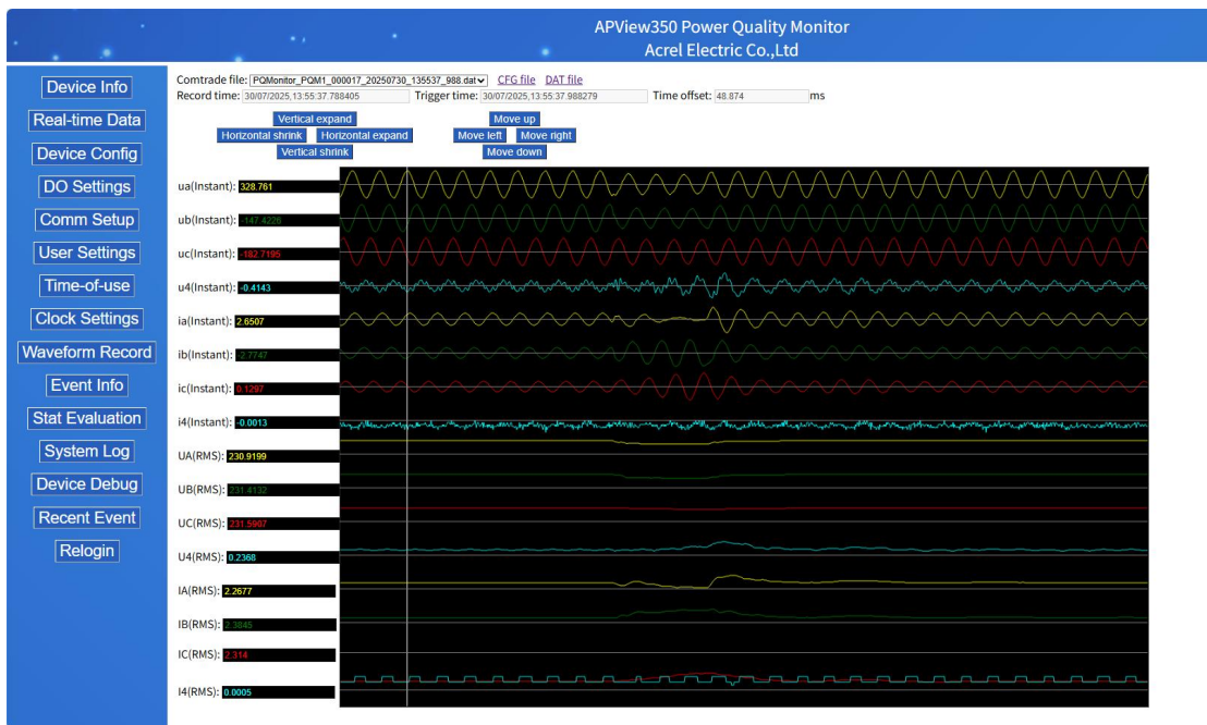
Fig. 1.5 Waveform Screen
