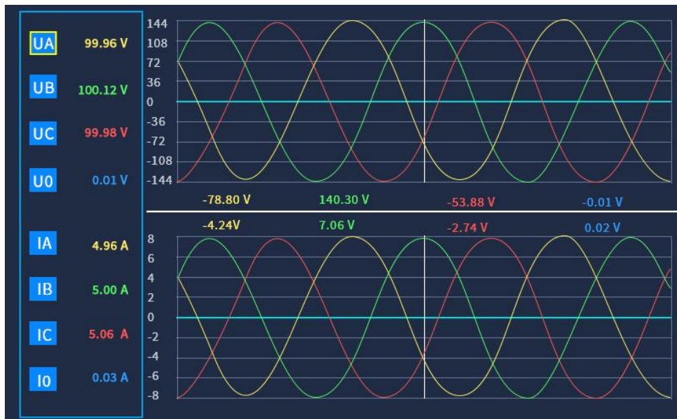
Fig. 4.7 Real-time Waveform
