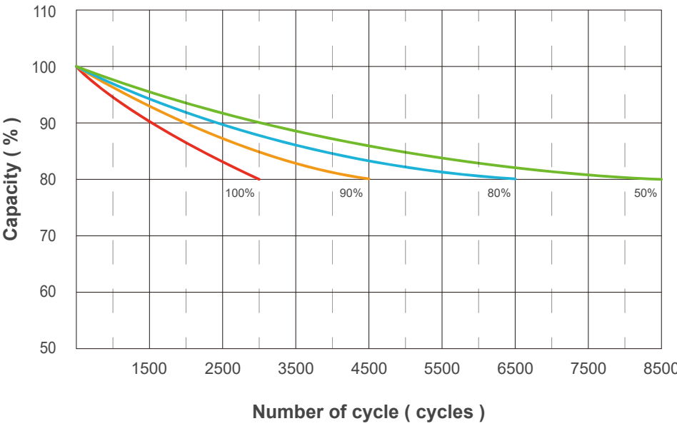
Cycle life with DOD at 25°C, 0.2C
