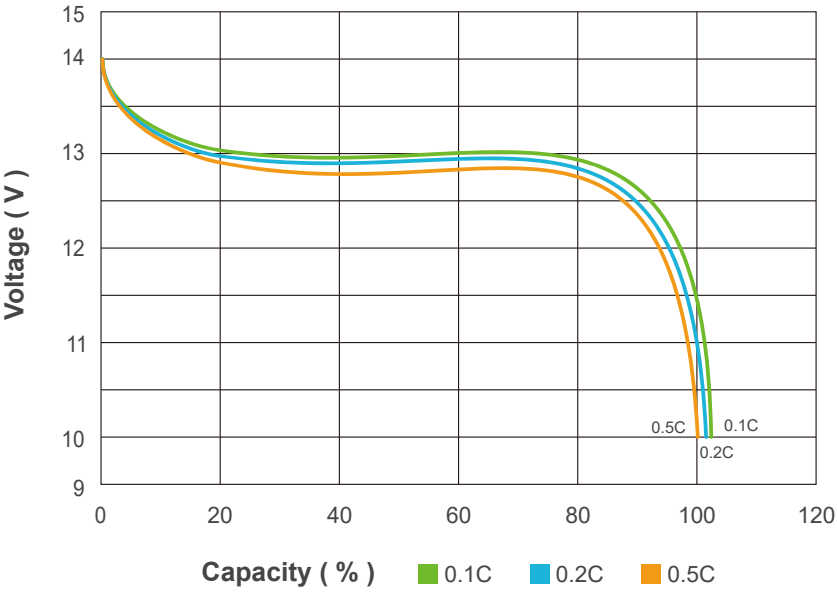
Discharge Performance at 25°C
