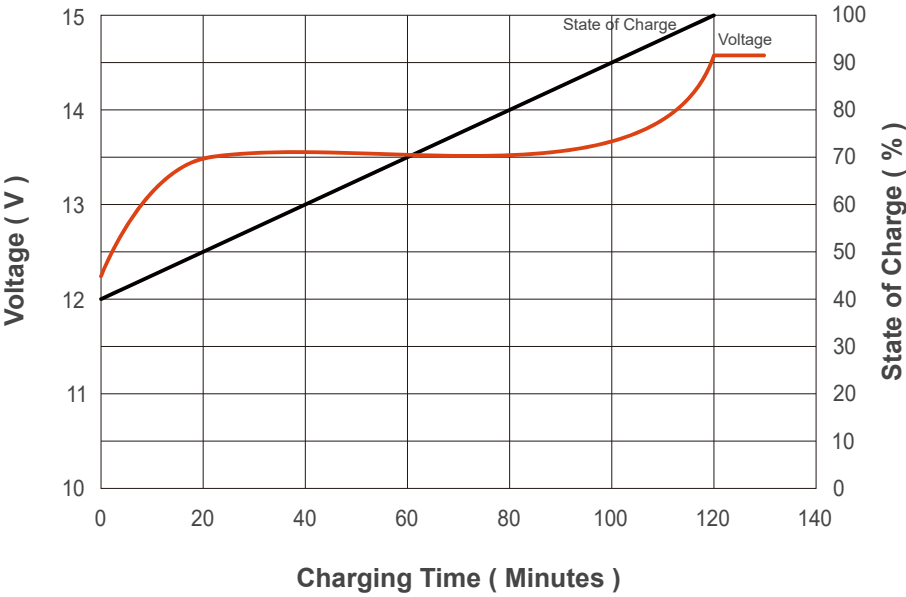
State of Charge Curve ( 0.5C, 25°C )
