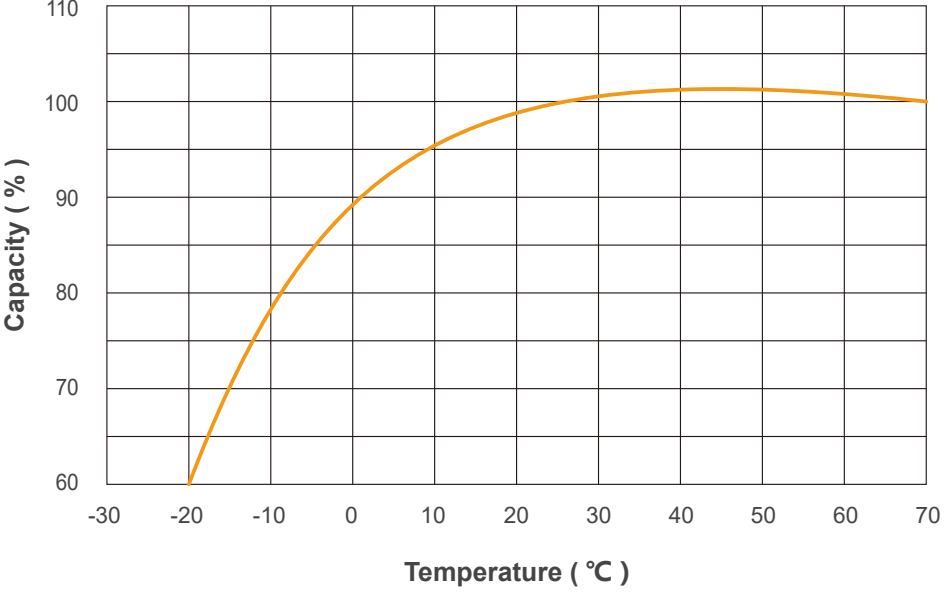
Temperature effects on capacity at 0.2C
