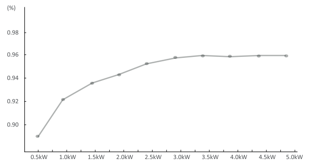
Battery - grid efficiency curve
