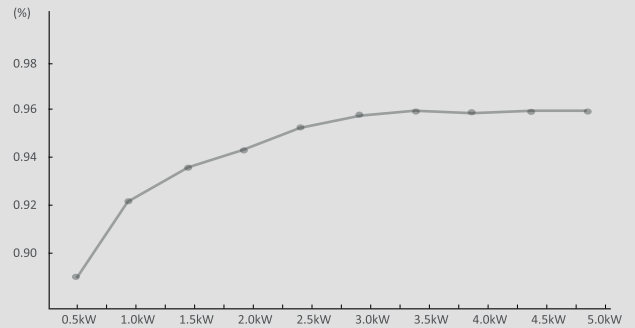
Battery - grid efficiency curve
