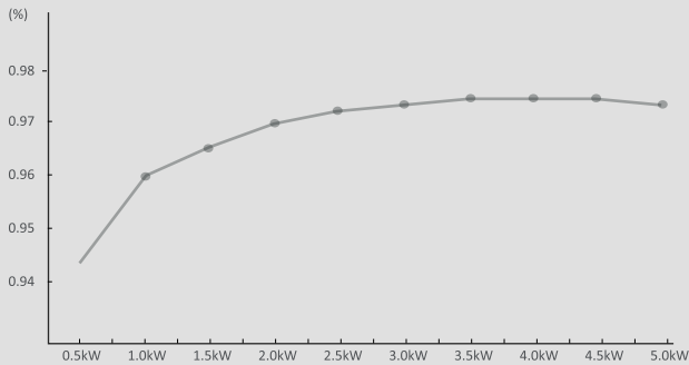
Photovoltaic - grid efficiency curve
